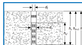
FIGURE 3 - Typical Installation Detail for Power-Sert for Internally Threaded Inserts
