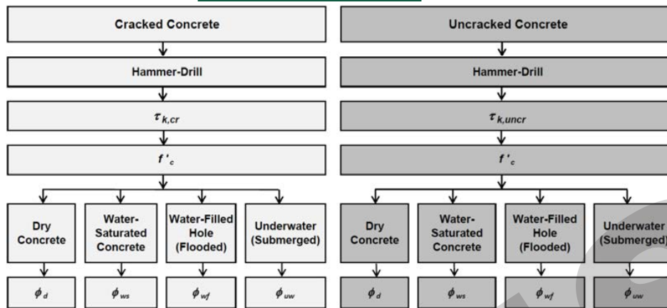
FIGURE 1—FLOWCHART FOR THE ESTABLISHMENT OF DESIGN BOND STRENGTH FOR POST-INSTALLED ADHESIVE ANCHORS
