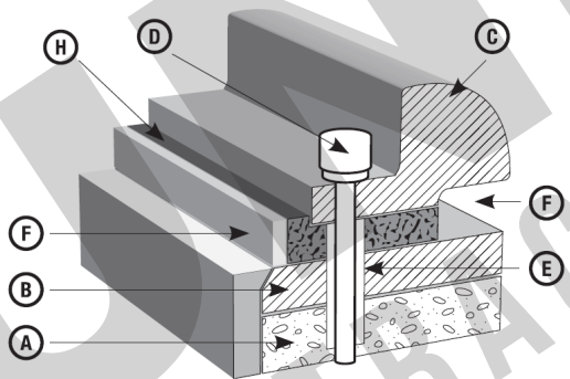
Figure 5 - Typical Epoxy Chock Application
