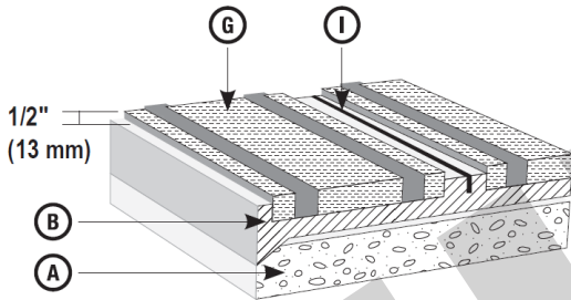
Figure 4 - Typical Rail with Expansion Joint Section
