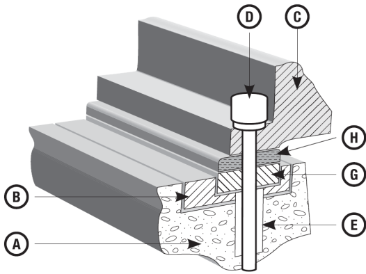
Figure 3 - Rail or Soleplate
