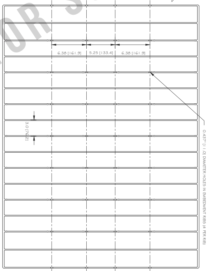
BOTTOM VIEW
