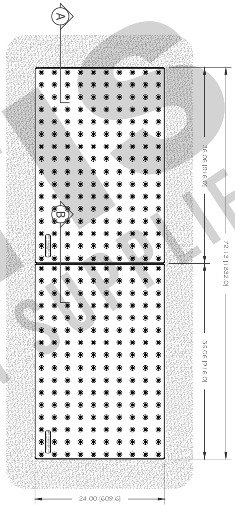
TOP VIEW - MULTIPLE PANEL INSTALLATION
