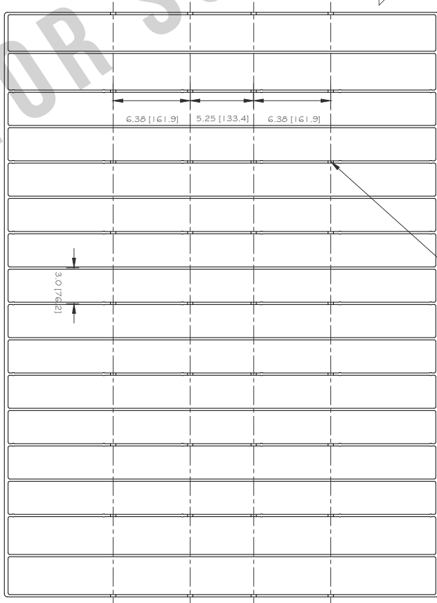
BOTTOM VIEW
