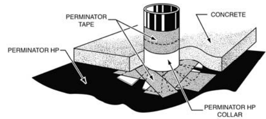
Figure 2: COLLAR INSTALLATION
